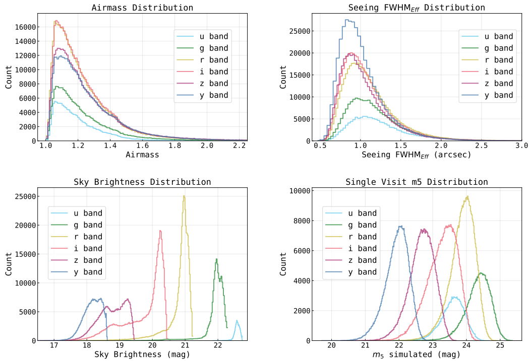
FIGURE 1: Distribution of airmass, seeing (FWHM Eff , see subsection 3.1), sky brightness, and m_5 for the 10-year LSST survey simulated in baseline_v2.0, including Wide-Fast-Deep and minisurveys within.
